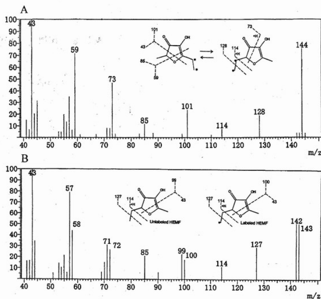
Fig. 2. GC-MS Data for HEMF Obtained by Incubation of Yeast with [U- ^{13}\text{C} ]-Glucose or [6- ^{13}\text{C} ]-Glucose Instead of the Corresponding Unlabeled Compound in the Basic Medium.
