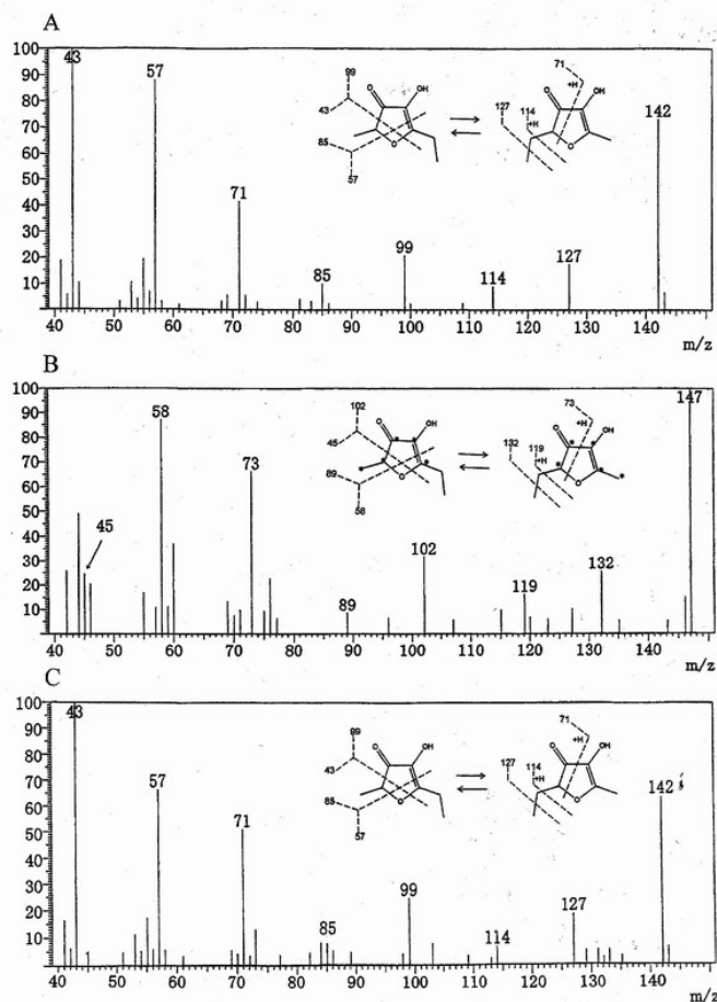
Fig. 1. GC-MS Data for HEMF Obtained by Incubation of Yeast with Normal Glucose, [U- ^{13}\text{C} ]-Ribose, or [U- ^{13}\text{C} ]-Glycine Instead of the Corresponding Unlabeled Compound in the Basic Medium.
